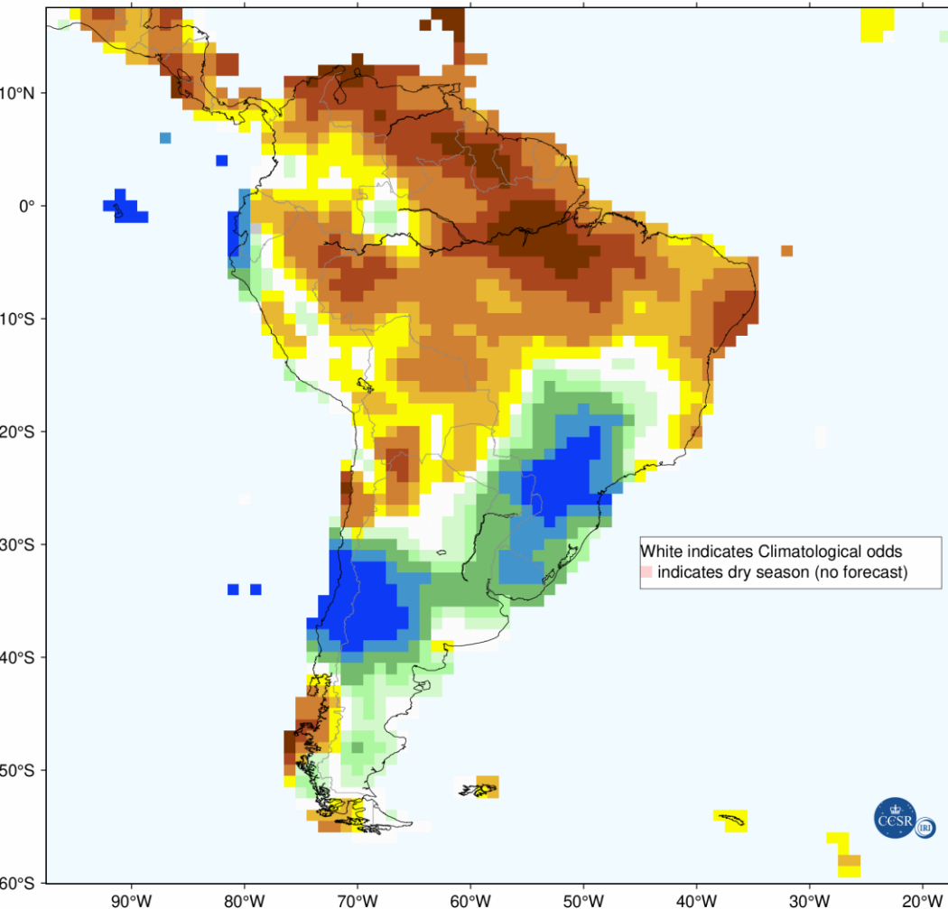
CCSR/IRI Multi-Model Forecast for Precipitation for September-October-November 2026, Issued August 2026
