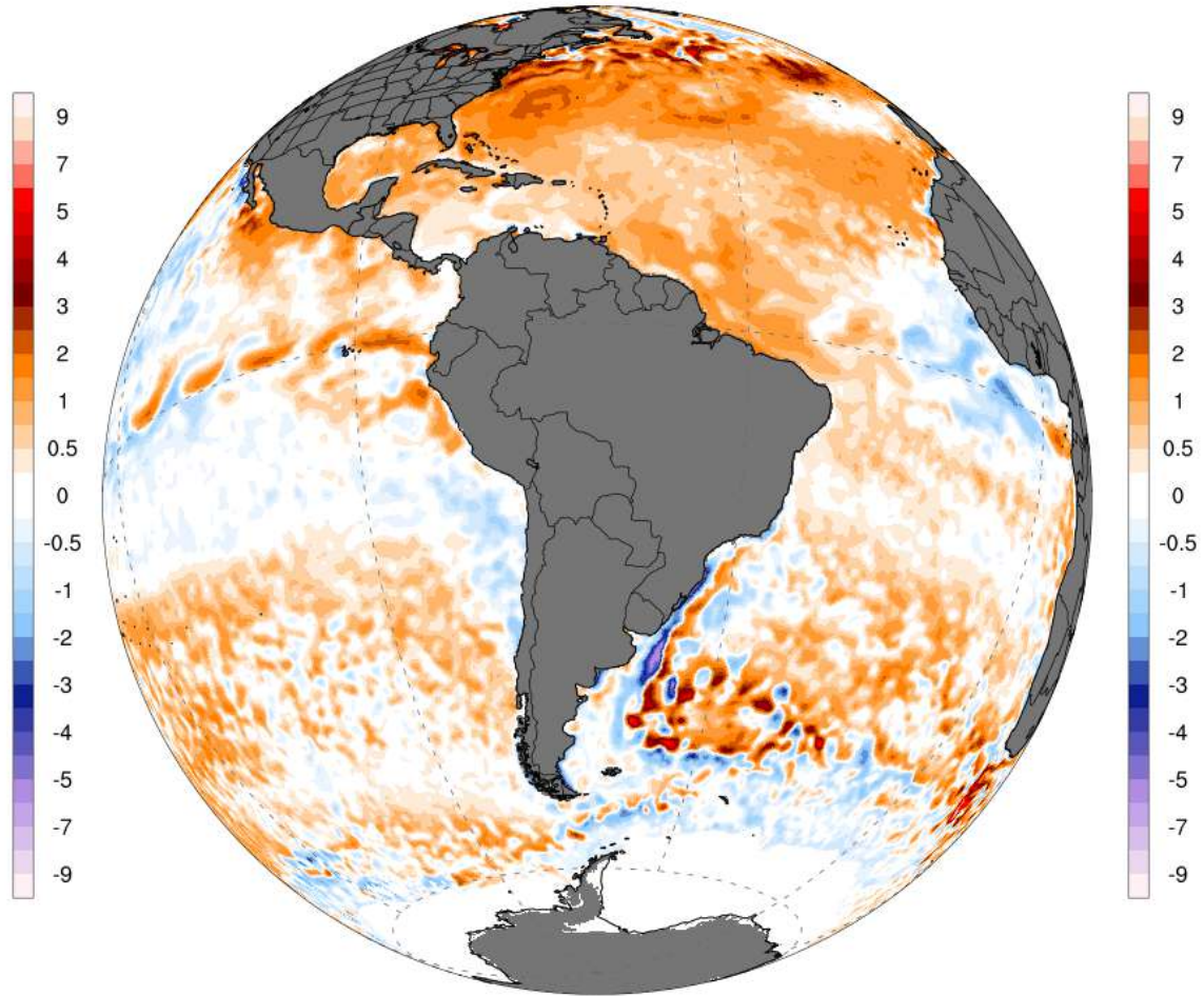
ClimateReanalyzer.org OISST SST Anomaly ( ^{\circ}\text{C} ) [1971-2000 baseline] Climate Change Institute | University of Maine 1-day Avg | Fri, Aug 01, 2025 [preliminary]
