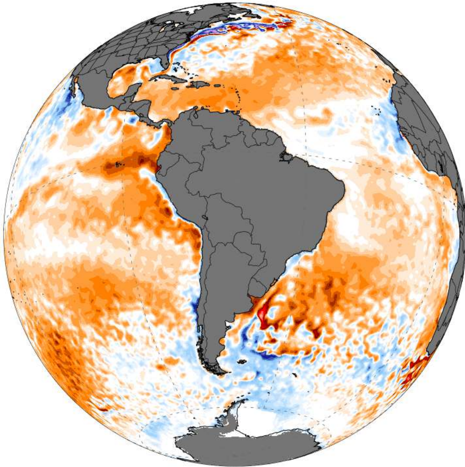
OISST SST Anomaly ( ^{\circ}\text{C} ) [1971-2000 baseline] 1-day Avg | Mon, Mar 24, 2025 [preliminary]
