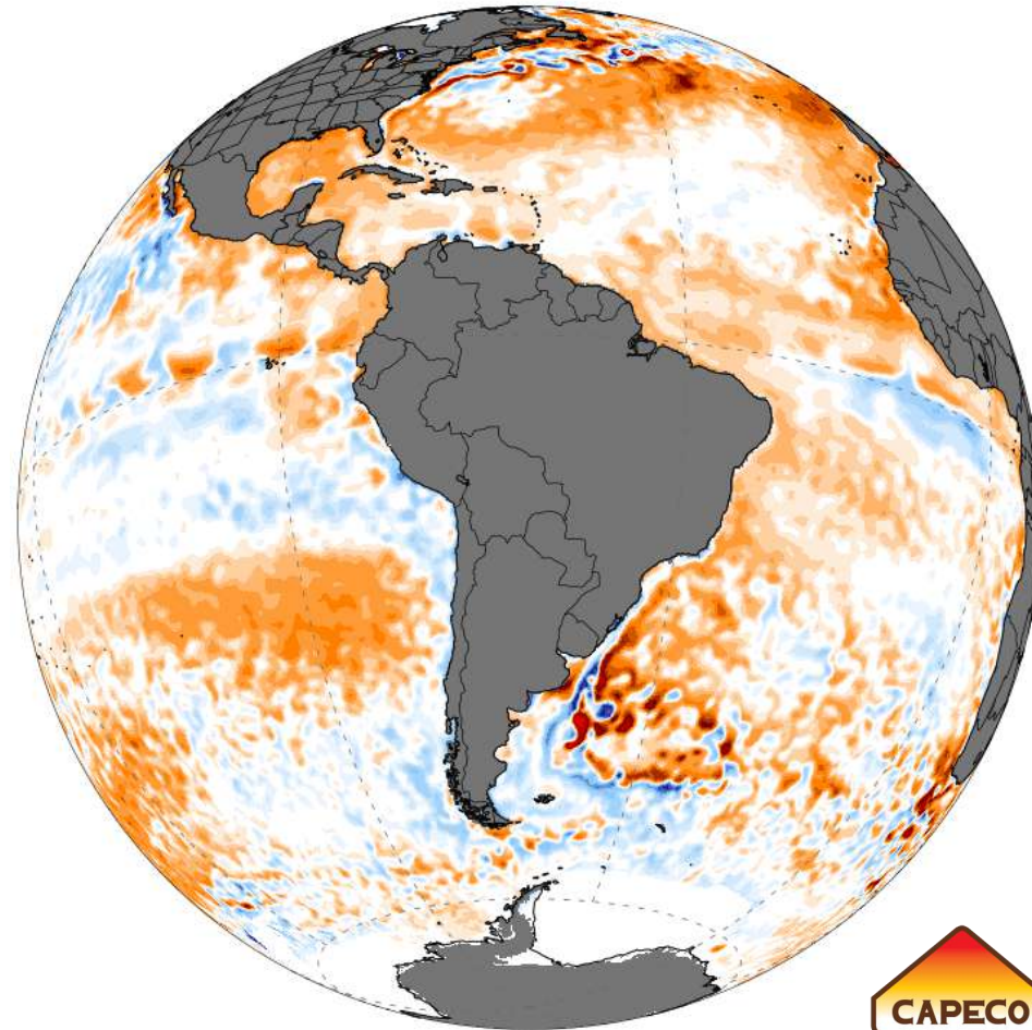
OISST SST Anomaly (°C) [1971-2000 baseline] 1-day Avg | Sun, Jun 08, 2025 [preliminary]
