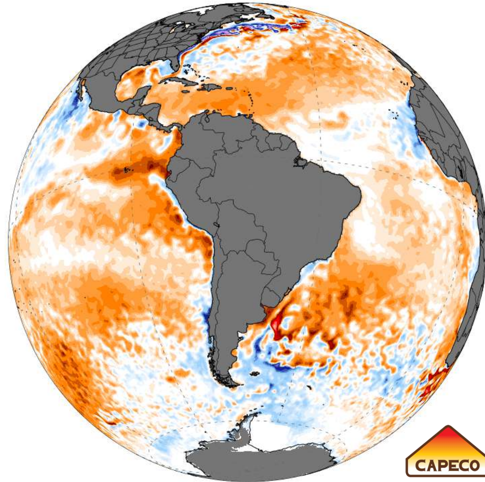
OISST SST Anomaly (°C) [1971-2000 baseline] 1-day Avg | Mon, Mar 24, 2025 [preliminary]
