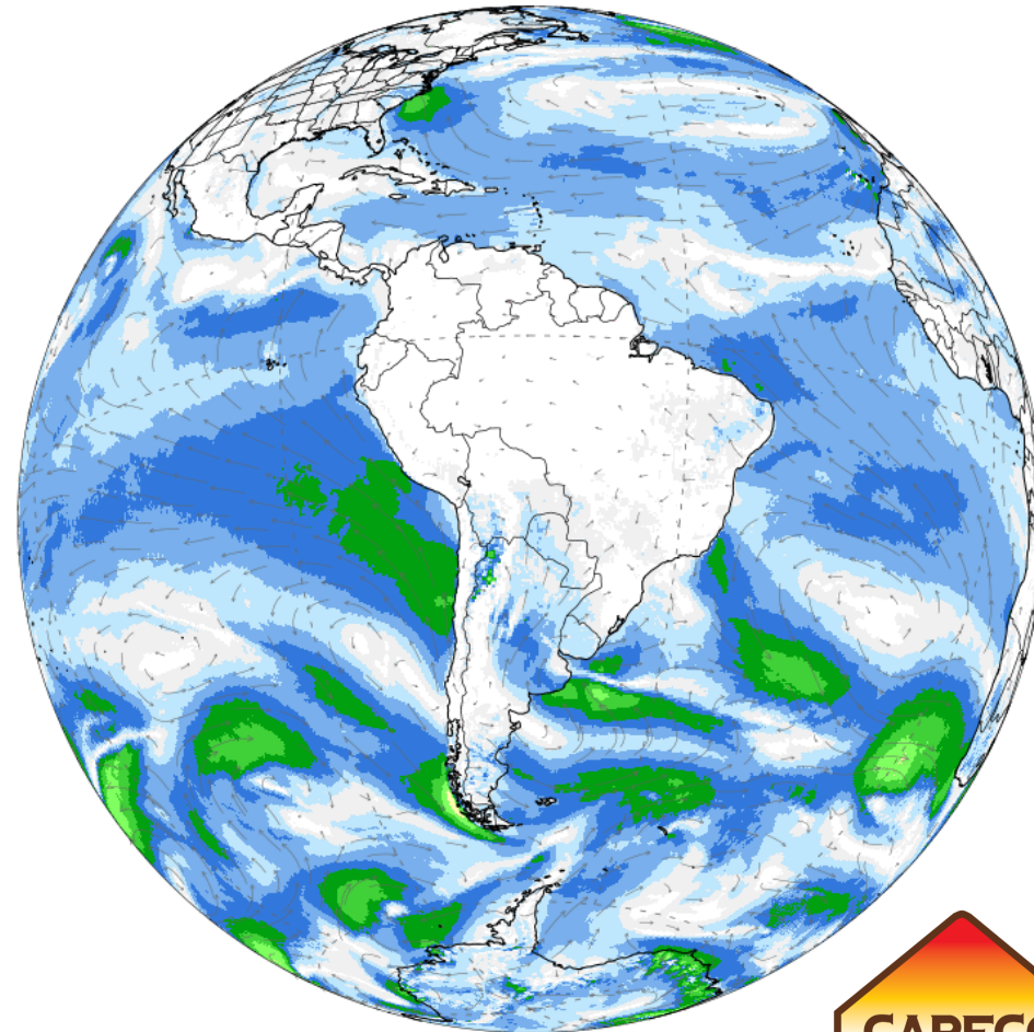
ClimateReanalyzer.org GFS 10m Wind Speed (kt) Climate Change Institute | University of Maine 1-day Avg | Thu, Aug 08, 2024
