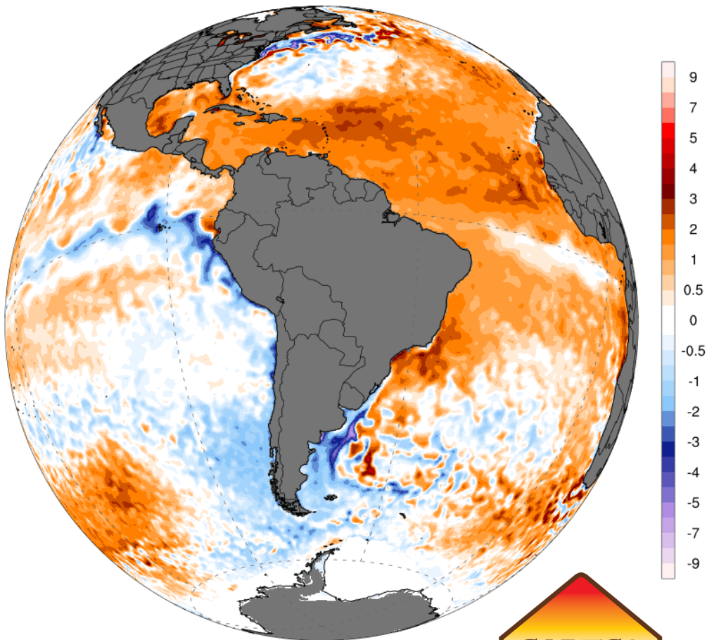
OISST SST Anomaly (°C) [1971-2000 baseline] 1-day Avg | Fri, May 17, 2024 [preliminary]
