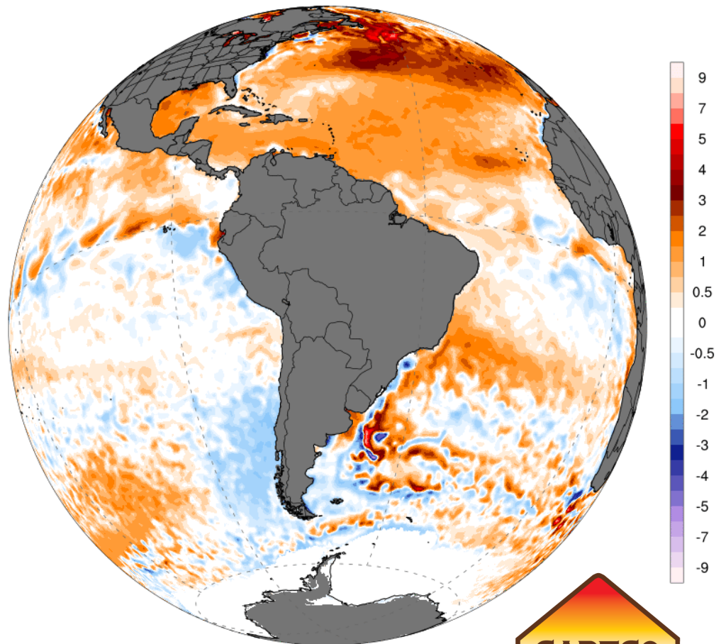
OISST SST Anomaly (°C) [1971-2000 baseline] 1-day Avg | Tue, Aug 06, 2024 [preliminary]
