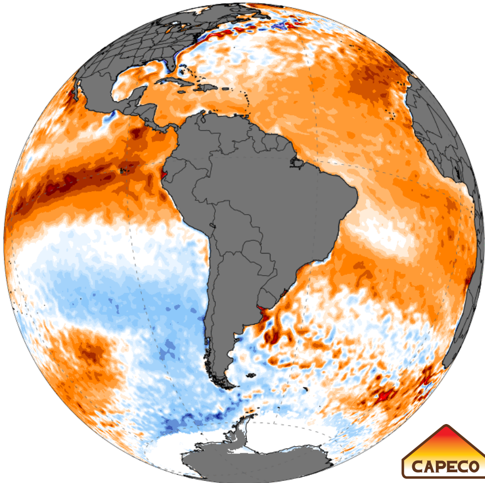
OISST SST Anomaly (°C) [1971-2000 baseline] 1-day Avg | Mon, Dec 18, 2023
