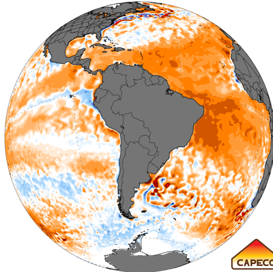
ClimateReanalyzer.org OISST SST Anomaly (°C) [1971-2000 baseline] Climate Change Institute | University of Maine 1-day Avg | Fri, Apr 12, 2024
