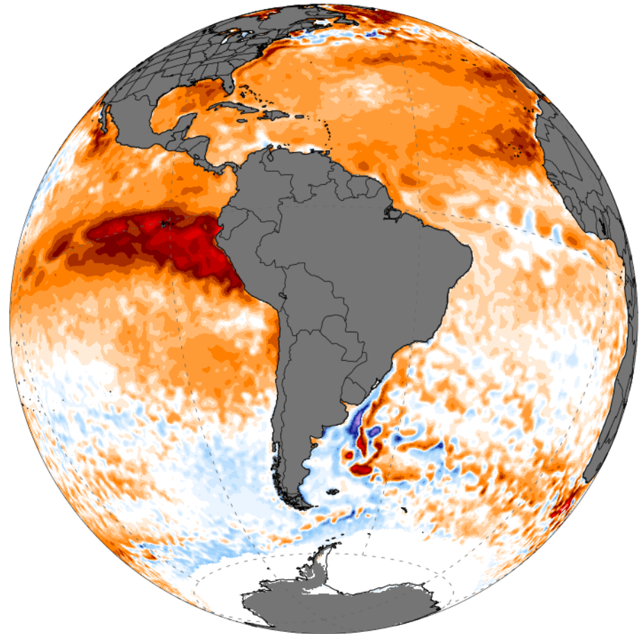
OISST SST Anomaly (°C) [1971-2000 baseline] 1-day Avg | Wed, Aug 16, 2023
